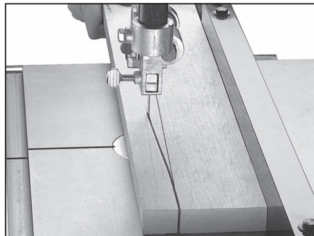
Figure 60. Example of blade lead.
