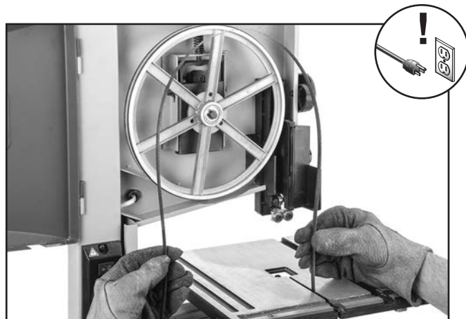
Figure 37. Example of removing blade.
