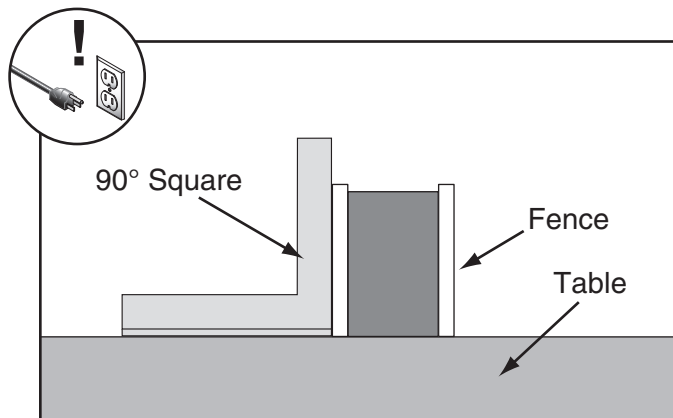
Figure 2. Example of checking fence squareness to table.
