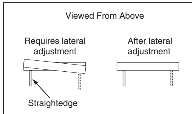
Figure 59. Before and after lateral wheel alignment (viewed from above).
