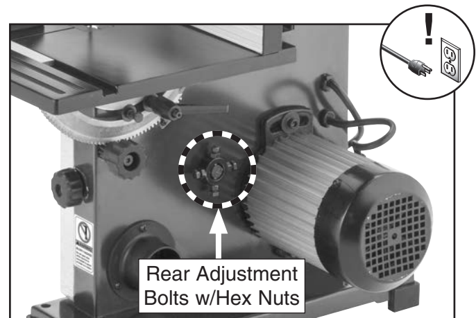
Figure 57. Location of rear lateral adjustment components.
