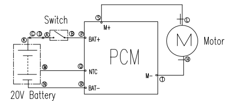
Electric Circuit
