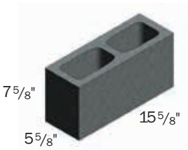
Partition Regular
