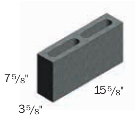
Partition Regular
