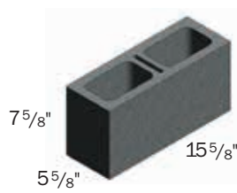
Partition Splittable
