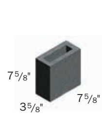
Half Partition
