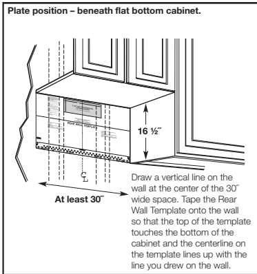
Plate position – beneath flat bottom cabinet.
