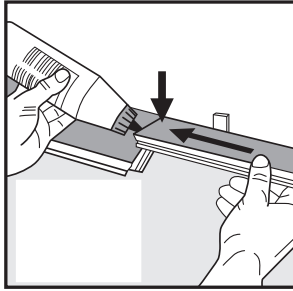
Fig. 2 Glue all of the short end joints in the first and last rows only. Use wood glue and weight down until glue has dried.
