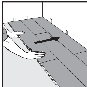
Fig. 12 After installing 2 rows, place the spacers along the wall, line up the boards on the chalk line and push the installed flooring rows against the spacers. Continue installing rows.
