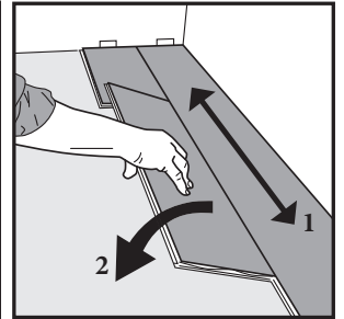
Fig. 10 Hint for installing planks. The long sides of planks must be fully aligned before rotating down. You cannot force the boards. If they are not lying flat, the long side is not fully engaged. Start over ensuring the long sides are fully engaged.
