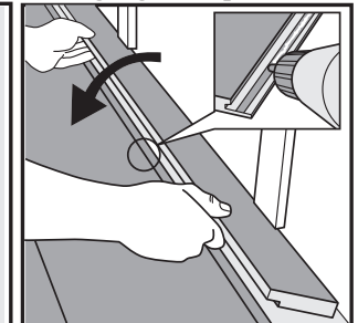
Fig. 15 Put glue along the modified locking profile, press the panels together and weight until glue is dry.
