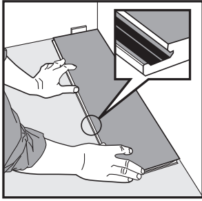
Fig. 1 First plank, first row. Start in the left-hand corner of the room with the groove side of the locking profile facing you. Use a spacer (equal to the thickness of the floor) between the left wall and the plank. The spacers between the long sides and the wall will be added after three rows have been installed.
