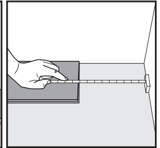
Fig. 5 At the end of the first row, put a 3/8" spacer along the wall, measure the length of the last plank to fit.
