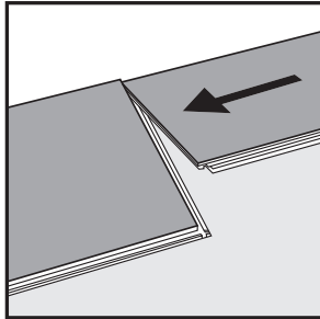
Fig. 3 Second plank, first row. Place next plank tight to the short end of the first plank.
