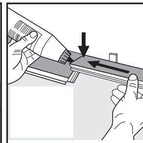
Fig. 13 Glue the short end joints in the last row and weight down until dry.
