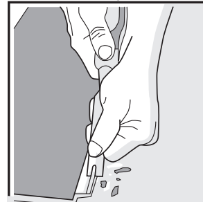
Fig. 14 Remove the raised portion of the groove using a chisel.
