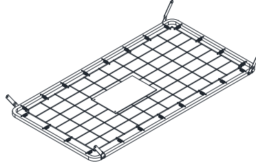
F. Mattress support (1 pc)
