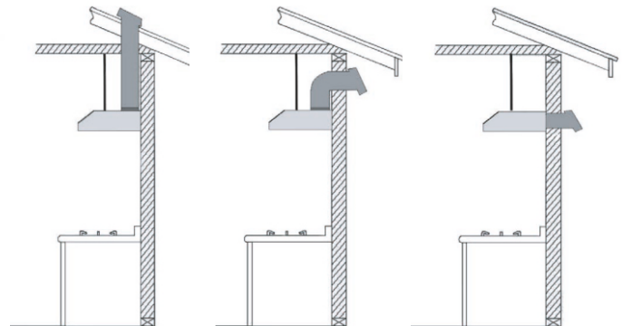
TOP VENTING ROOF EXHAUST
