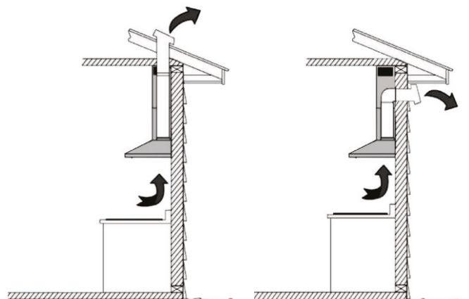
TOP VENTING ROOF EXHAUST
