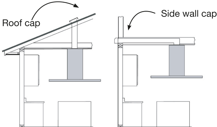
TOP VENTING ROOF EXHAUST
