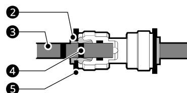
2 Collet 3 Tube 4 Insert line 5 Clip
