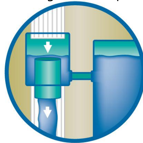
(2) Rain barrel is Full, Diverting to Downspout
