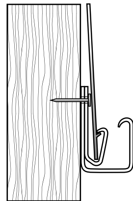
Fig. 3 J-Channel and Undersill Trim
