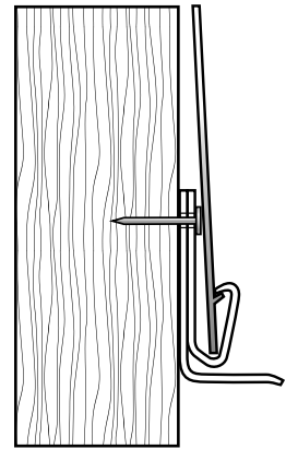
Fig. 2 Undersill with Snaplock and Flashing
