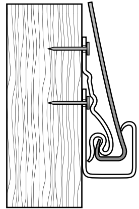
Fig. 1 Starter Strip Inside J-Channel
