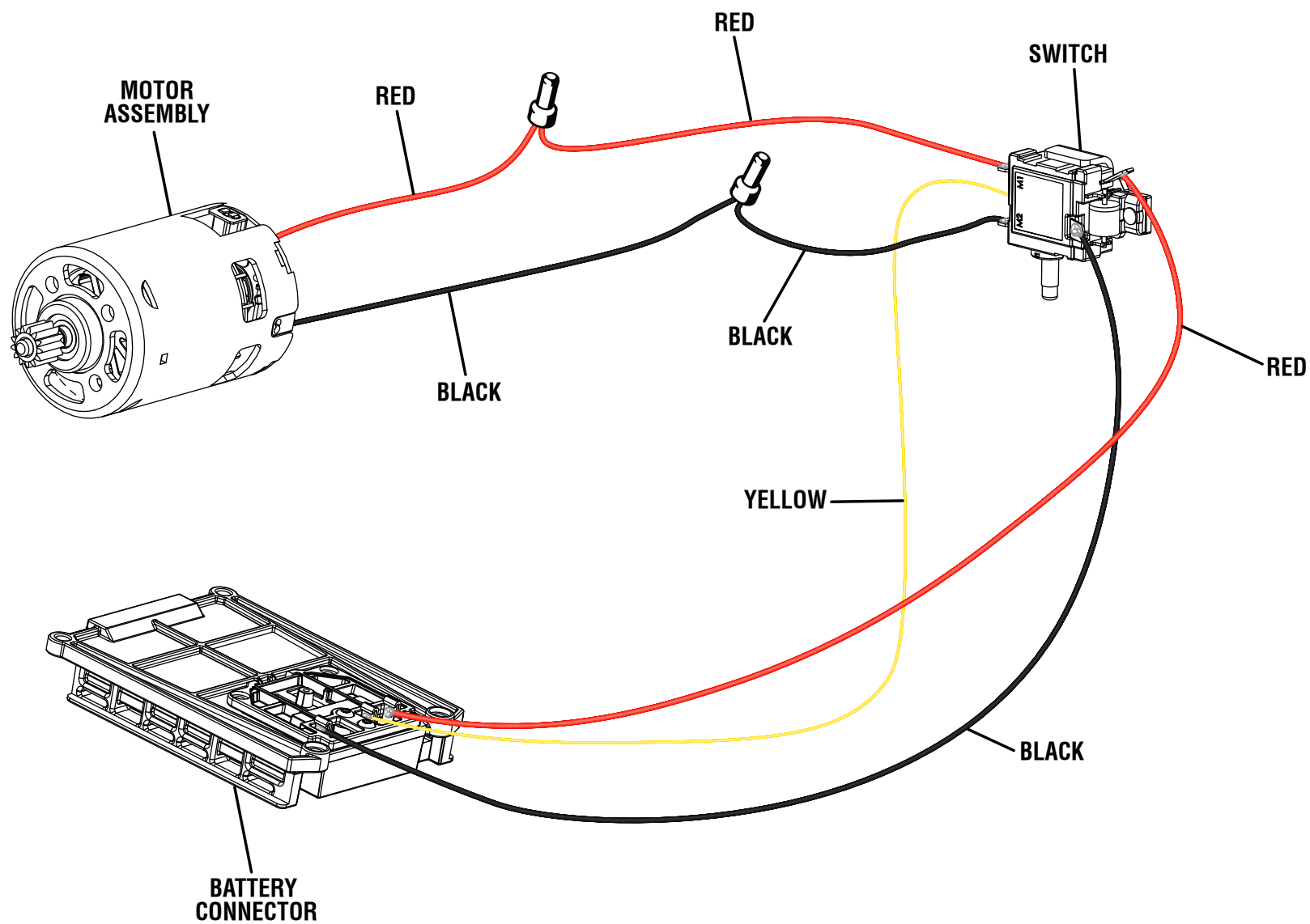
WIRING DIAGRAM
