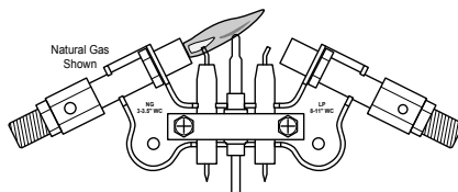
Figure 22 - Correct Pilot Flame Pattern
