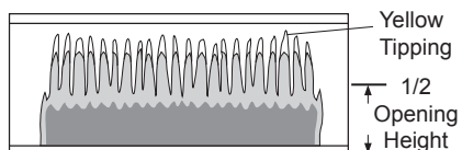
Figure 25 - Incorrect Burner Flame Pattern
