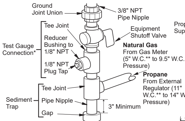
Figure 15 - Gas Connection
