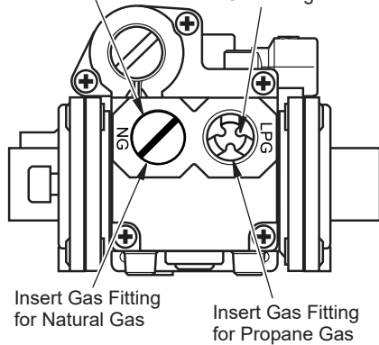
Figure 14 - Gas Regulator
