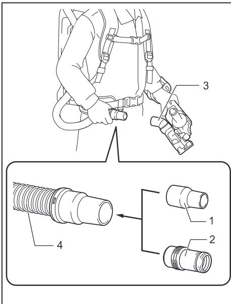
► 1. Joint 2. Front cuff 3. Extraction outlet 4. Hose
