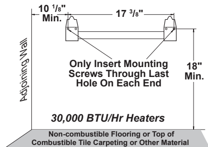
Figure 7 - Mounting Bracket Clearances
