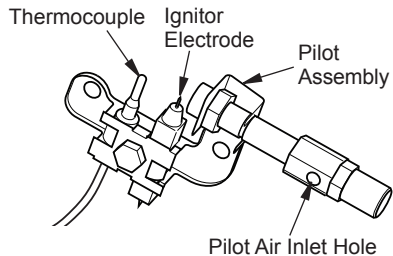
Figure 25 - Pilot Inlet Air Hole
