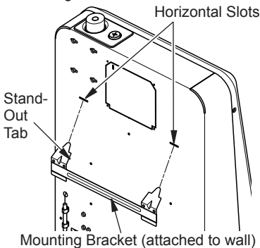
Figure 10 - Mounting Heater Onto Mounting Bracket
