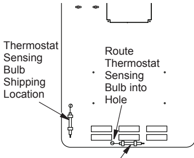
Figure 6 - Moving Thermostat Sensing Bulb
