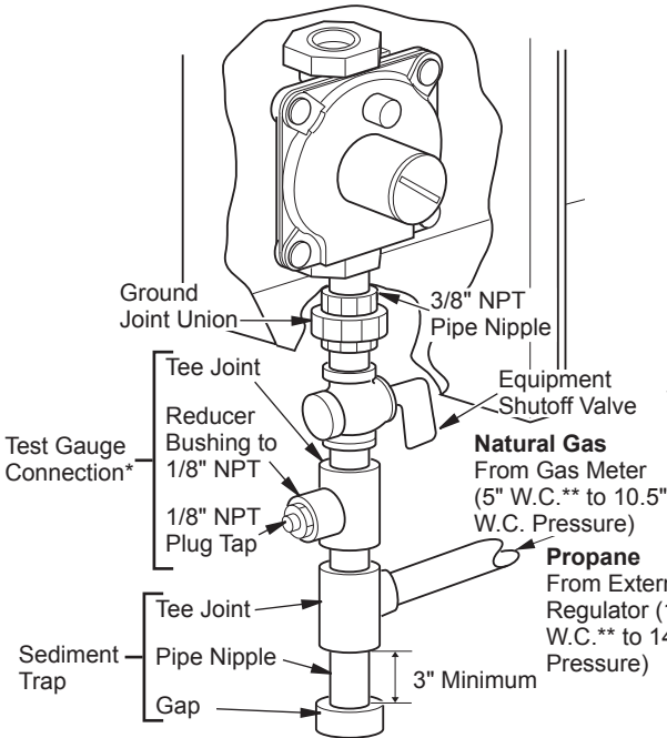
Figure 12 - Gas Connection
