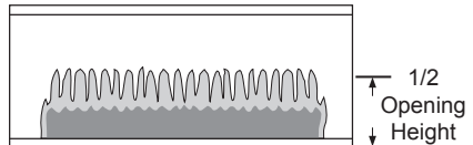
Figure 23 - Correct Burner Flame Pattern
