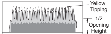
Figure 24 - Incorrect Burner Flame Pattern
