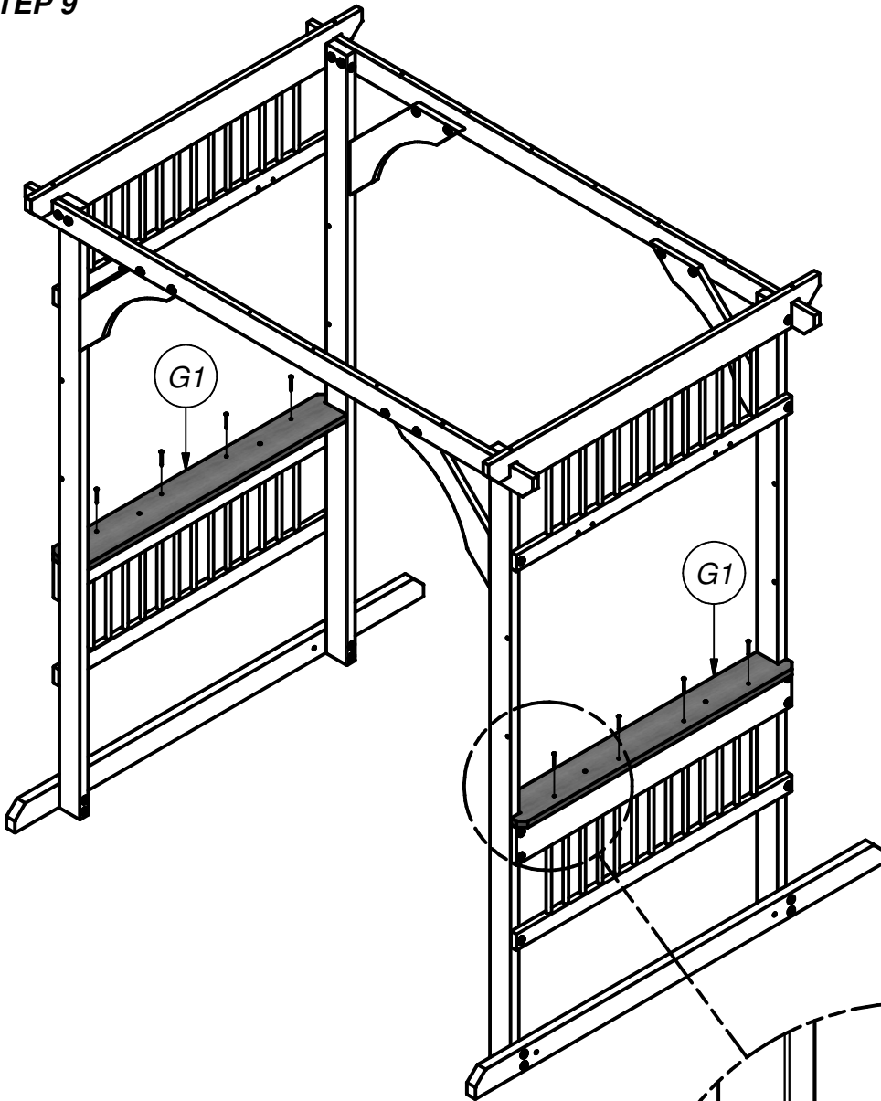
(2) G1 - SHELF - W4L05459 1"x5 1/4"x44 1/2" (24x134x1130)
