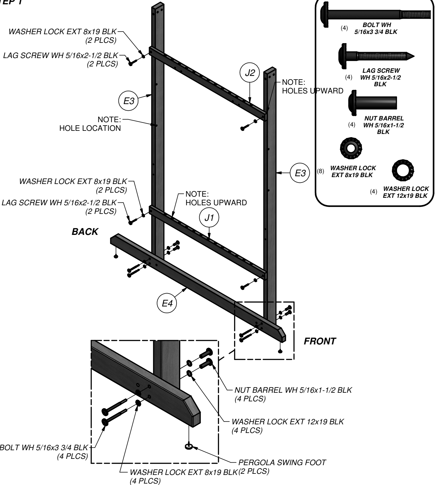
(2) - PERGOLA SWING FOOT - A6P00081
