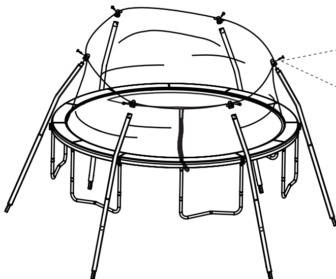
14 M5x44mm Bolt (x6)
