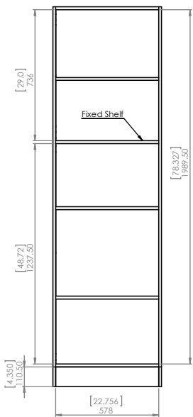
Front View (front door removed)
