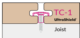
TC-1 (Locking Clip)
