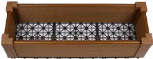
Planter Box QD-PB-13 (36" x 12" x 8-3/4") 15 lb/set
