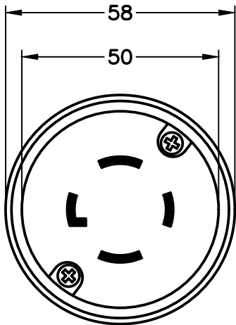
NEMA L14-30 PLUG FRONT VIEW
