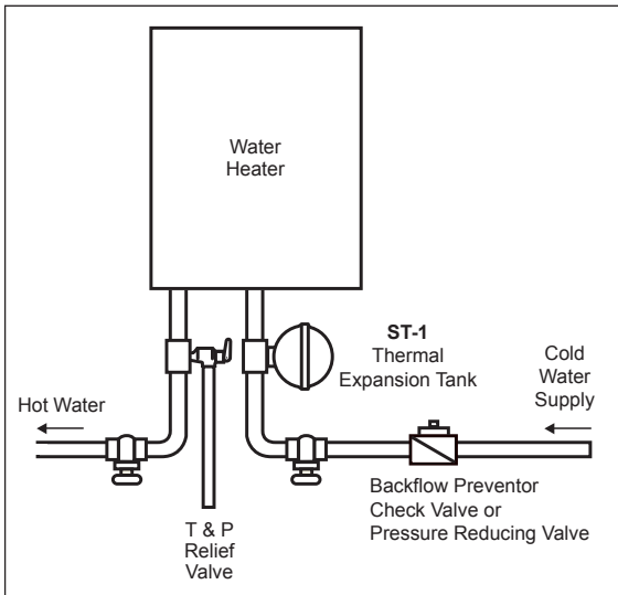
Figure 1. Typical Installation
