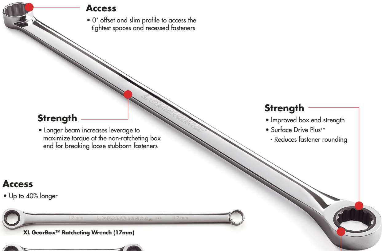
Double Box Ratcheting Wrench (17mm)
