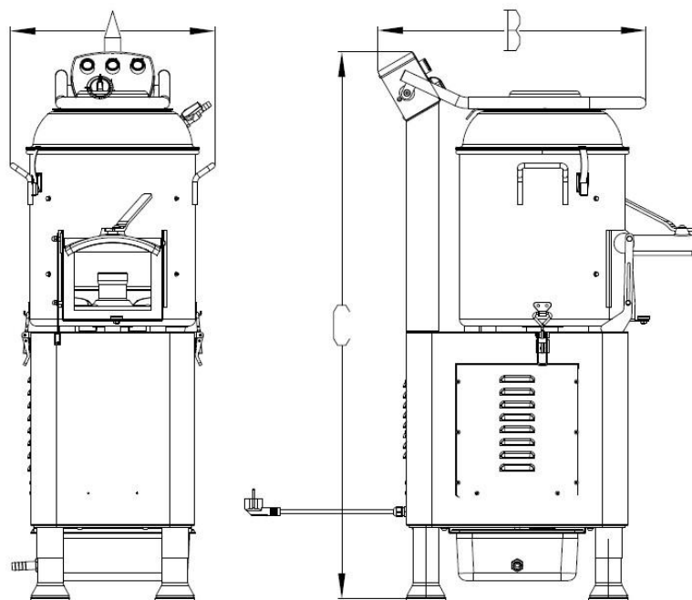
FIG.n ° 2—Drawings of dimensions
