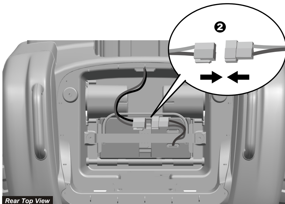
Rear Top View
