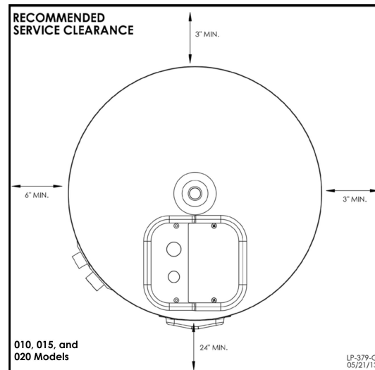
Figure 1 - Recommended Service Clearances
