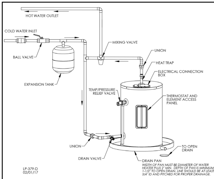
Figure 4 - Piping Detail - NOTE: Drawing is meant only to demonstrate system piping concept. The installer is responsible for equipment and detailing required by local codes.
