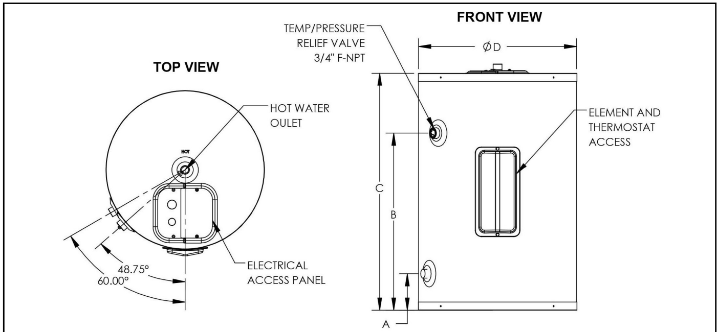
Figure 2 - Dimensional Drawing
