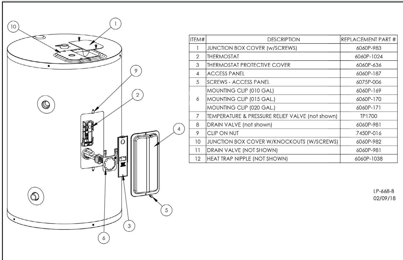
Figure 10 - Replacement Parts
