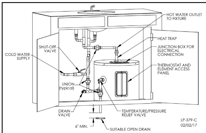
Figure 6 - Point of Use Installation - NOTE: Drawing is meant only to demonstrate system piping concept.
