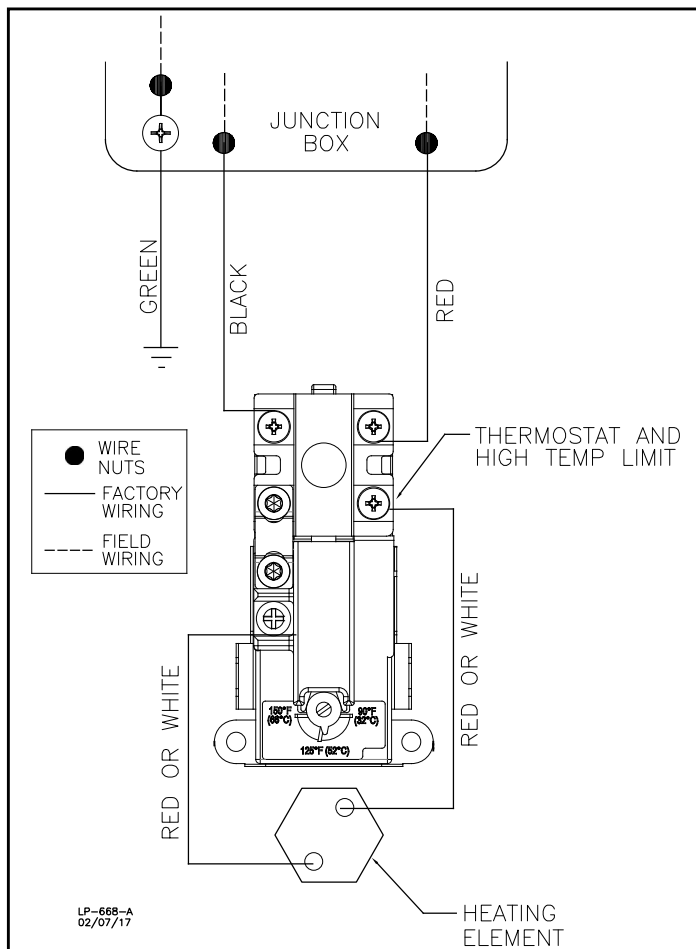
Figure 7 - Single Element Model Wiring Detail
