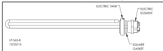
Figure 9 - Heating Element Detail
