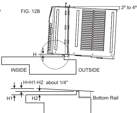
Vinyl-Clad Window
