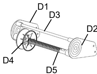
D. Hose guide device including:
