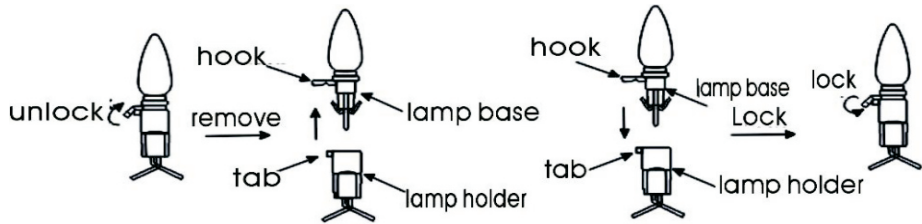
Fig.1 Unlock and remove the burned out lamp
