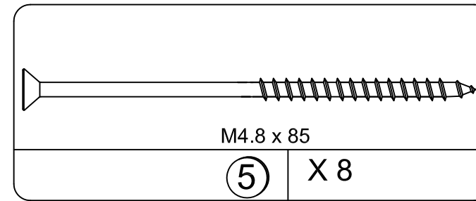
SCREW TTL1075
