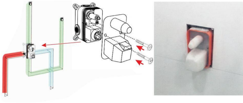
A:Wall Mounted Installation
