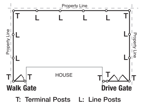
Sample Fence Layout
