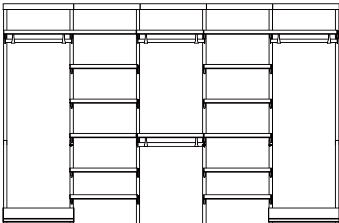
121.5 in. Long Hang and Double Hang with Double Six Shelf Stacks and Shoe Rack
