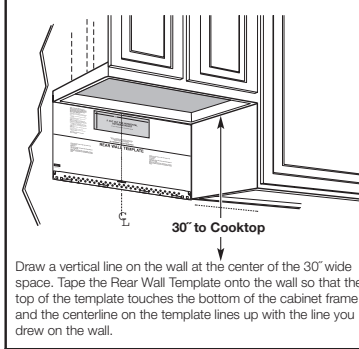
Plate position – beneath framed recessed cabinet bottom.
