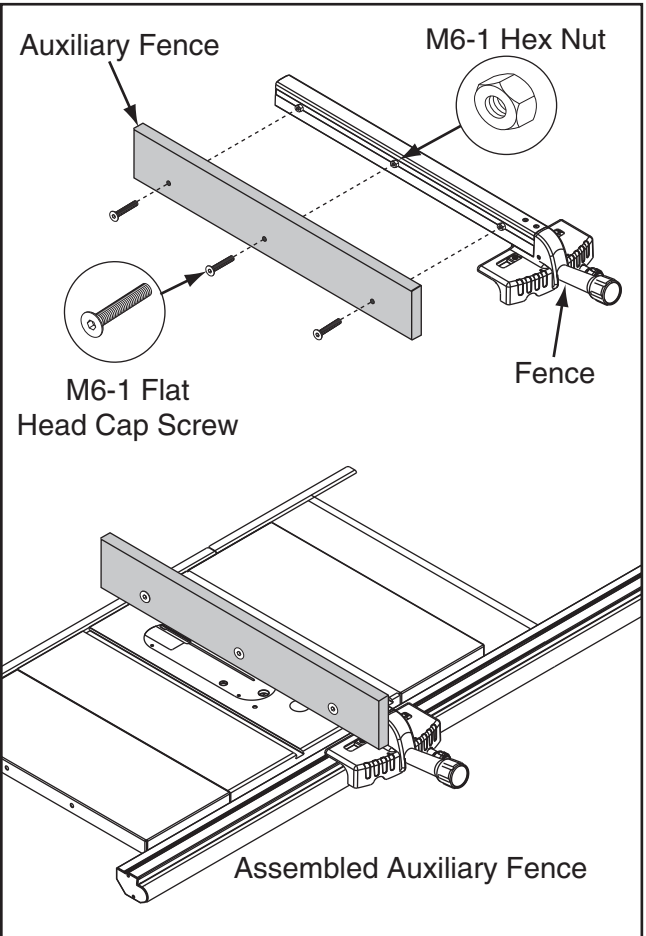
Figure 69. Example of auxiliary fence attached to Model G0771Z fence face.
