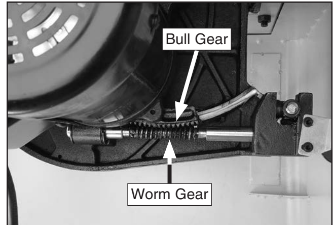
Figure 103. Worm and bull gear.
