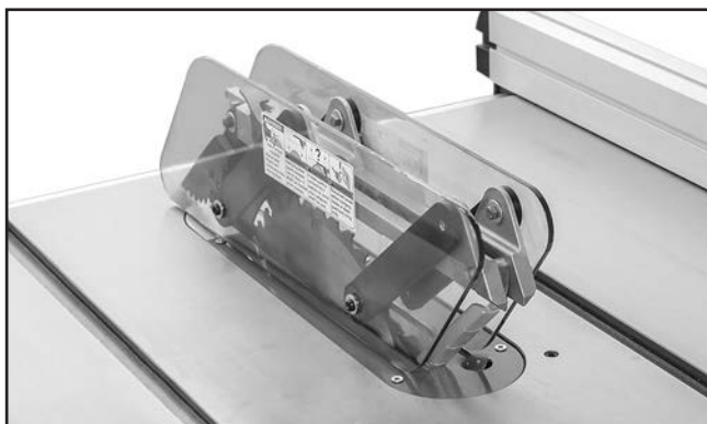
Figure 48. Blade guard installed.
