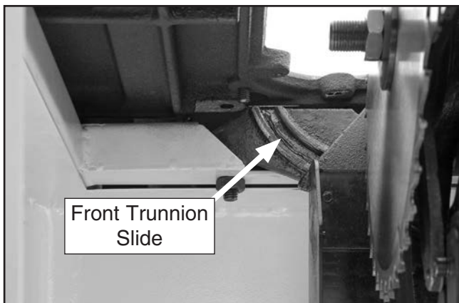
Figure 102. Trunnion slide (only front slide shown).
