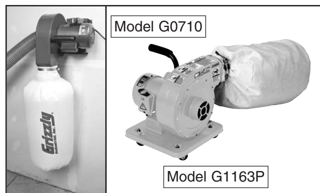
Figure 95. Point-of-use dust collectors.
