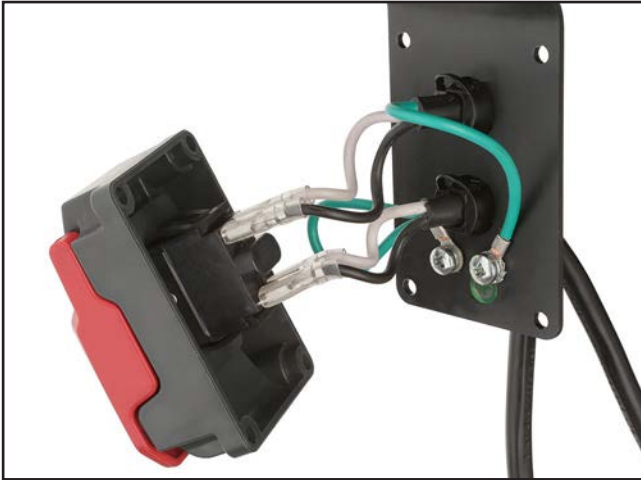
Figure 132. Switch wiring.
