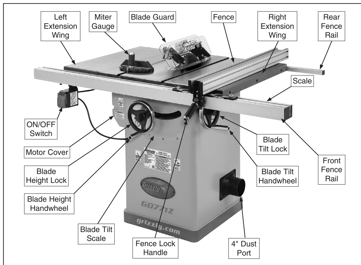
Figure 1. Model G0771Z identification of main controls and components.
