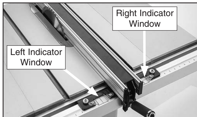
Figure 127. Fence indicator windows.
