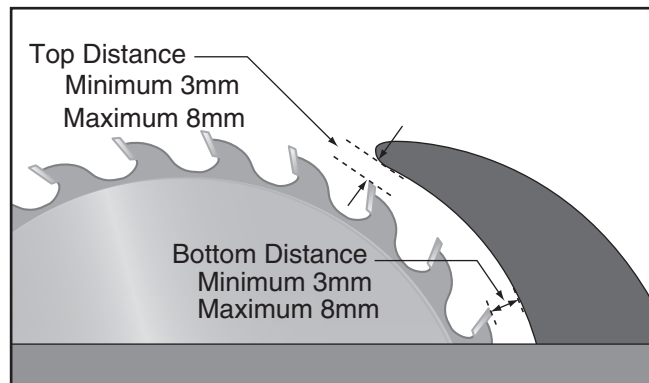
Figure 53. Example of allowable top and bottom distances between riving knife and blade.
