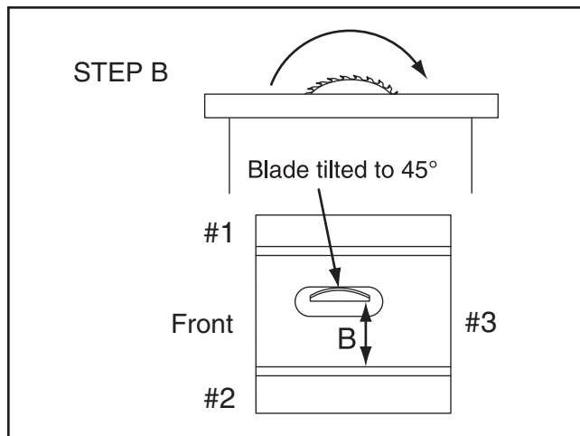
Figure 114. Shim procedure diagram B.
