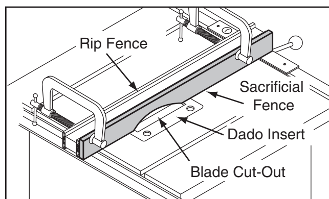
Figure 64. Example of sacrificial fence.
