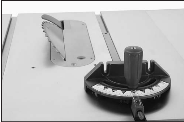
Figure 58. Example of blade tilted to 45° for bevel cutting (blade guard only removed for clarity).
