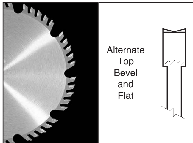
Figure 40. Combination blade.
