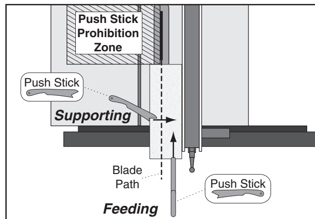
Figure 80. Using push sticks to rip narrow stock.
