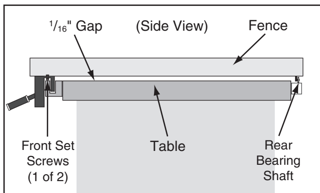
Figure 119. Fence height is adjusted by two front set screws and rear bearing shaft.
