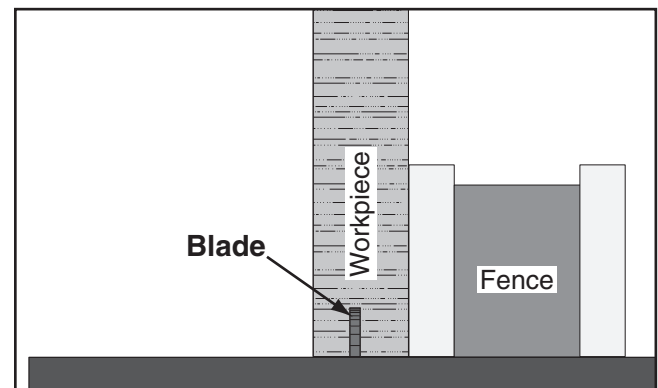
Figure 66. Example of rabbet cutting with a standard blade.
