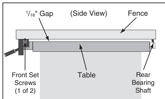
Figure 121. Example of even gap between fence and table approximately \frac{1}{16} " front to back.
