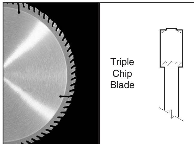
Figure 41. Laminate blade.
