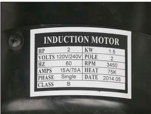
Figure 134. Motor label.
