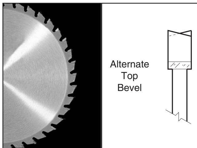
Figure 39. Crosscutting blade.
