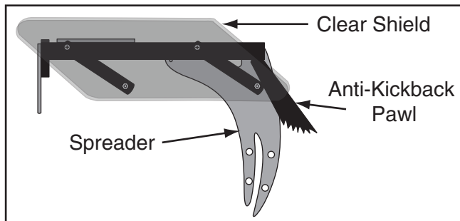
Figure 45. Blade guard assembly components.
