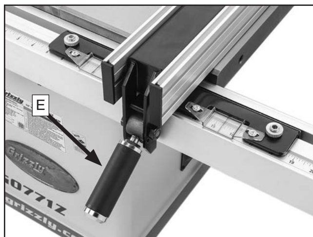
Figure 4. Fence lock handle.
