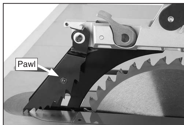
Figure 50. Pawls in resting position.
