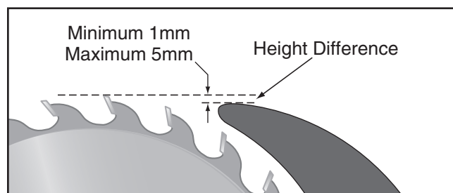
Figure 52. Example of height difference between riving knife and blade.
