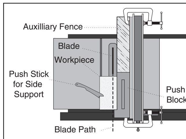
Figure 90. Push block in position to push workpiece through blade.
