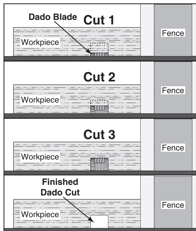
Figure 60. Example of dado being cut with multiple light cuts, instead of one deep cut.
