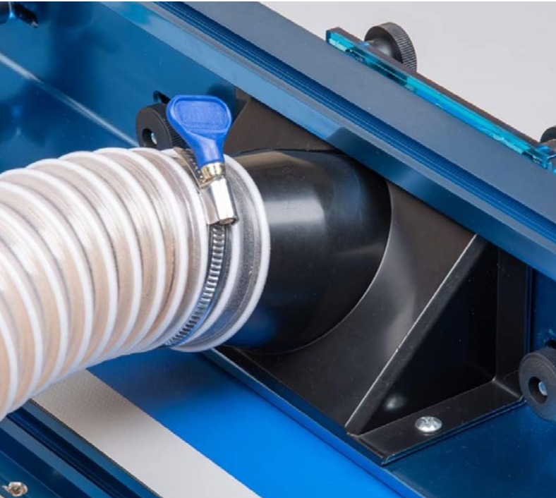
70243 2-1/2" 20 Feet Flexible PVC Dust Collection Hose with 2 Key Hose Clamps
