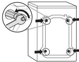
Unpacking and removing shipping bolts
