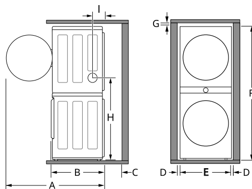
Dimensions and Clearances
