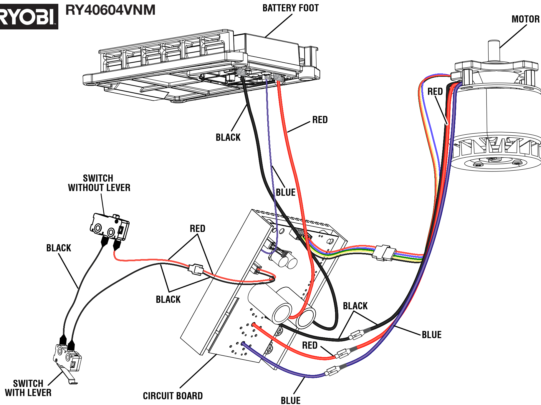
WIRING DIAGRAM
