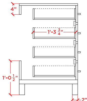
BASE CABINET SIDE VIEW
