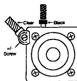
(2192) Fountain Air Valve Configuration Only
