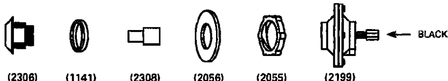
Assembly NO: 2199-C (Used only on FP Fountains: Pipe Ftn.s. Also used on all Pipe Showers, Push Button Jug Fillers & Mistlers)
