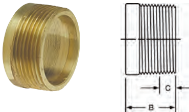
802-C ⚠ DWV Flush Adapter C x M – Cast
