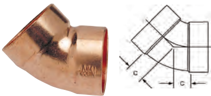
906 DWV 45° Elbow C x C – Wrot
