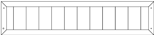
WP03 WALL PANEL - W2A03786 (x1) 1"x18 7/8"x11 3/4" (24x214x971)
