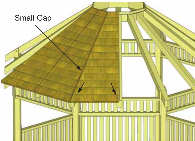
71. Position and attach as per Step 66 - 67 . Use 2 - 3" screws in Corner Rafter and Mid Rafter through bottom row of shingles. Lift and position 2nd Right Side Roof Panel on Center and Corner Rafter.
