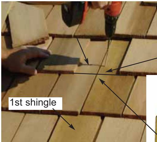
117. With a 3" screw, secure Roof Panel down into Mid Rafter above Exposure line. Screw both left and right Roof Panels down to Mid Rafters. Make sure to screw into rafter above the exposure line to conceal screw.
