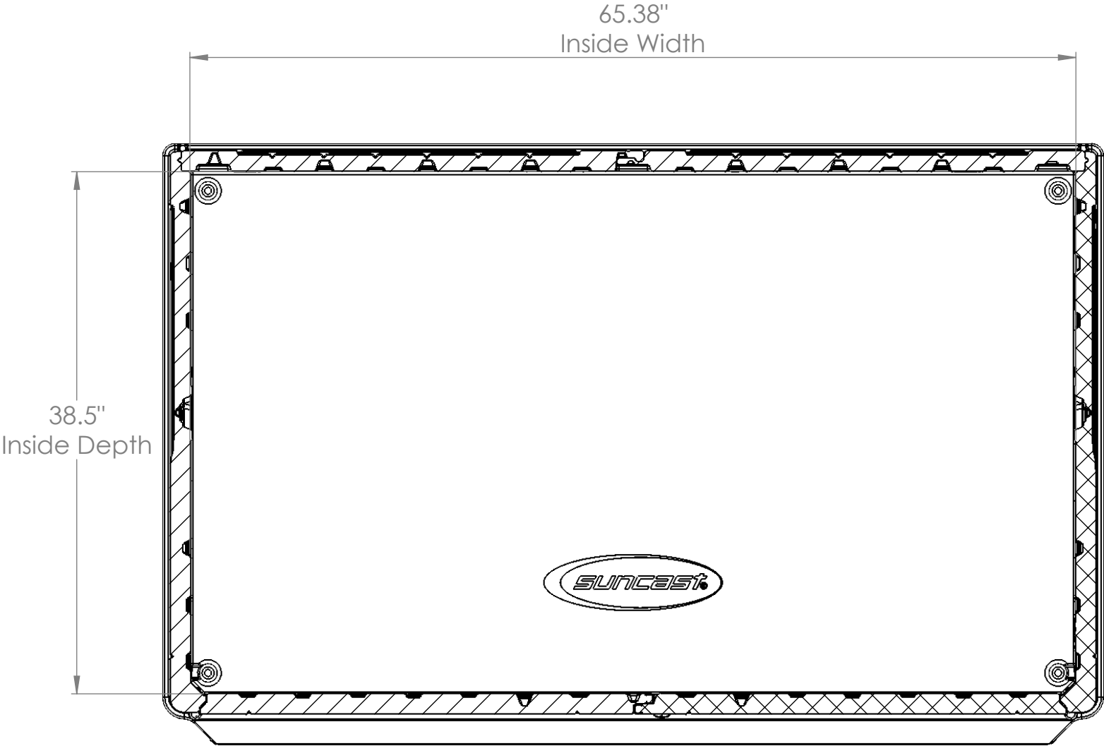
SECTION B-B
