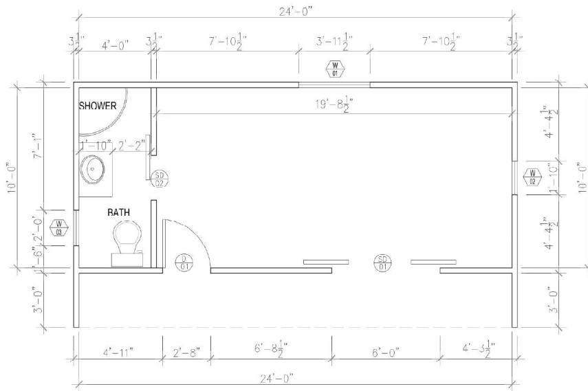
1 GROUND FLOOR PLAN Scale 1"=1/4"
