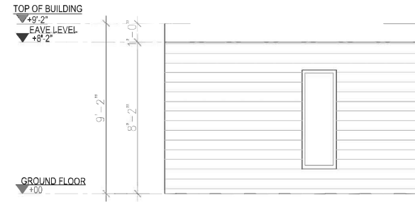
4 LEFT SIDE ELEVATION Scale 1"=1/4"
