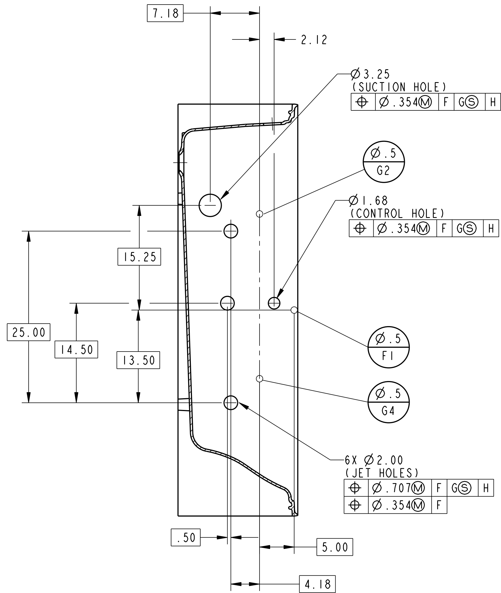
SECTION K-K
