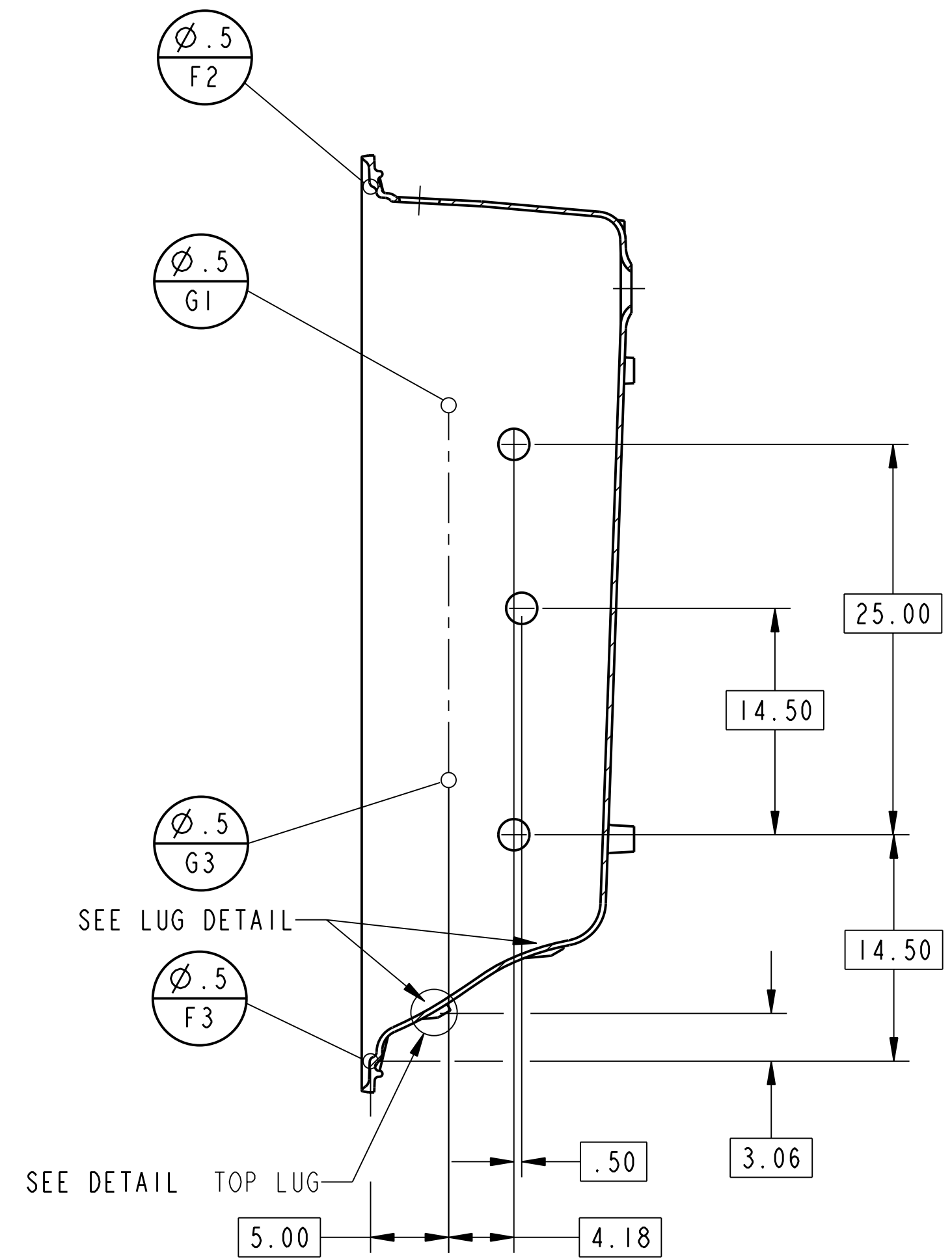
SECTION L-L
