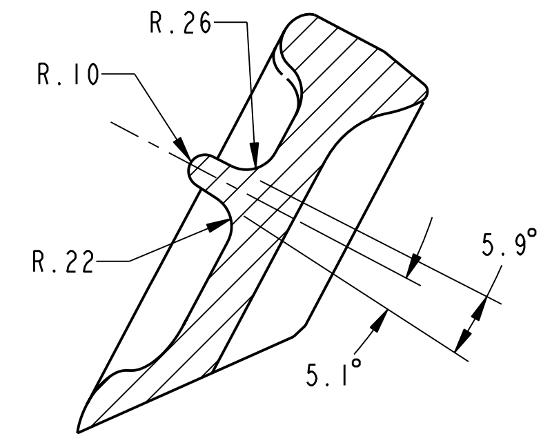
SECTION J-J SCALE 1.000
