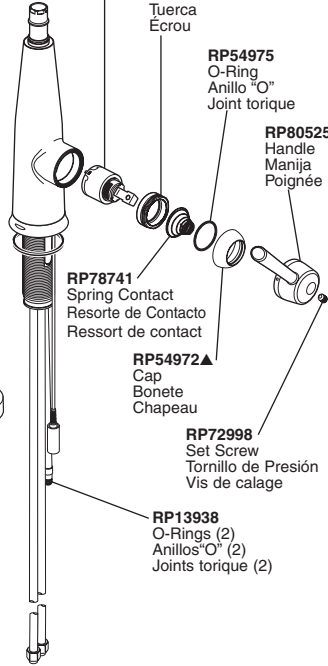
RP74836 Cartridge Assembly Ensamble del la Válvula Soupape
