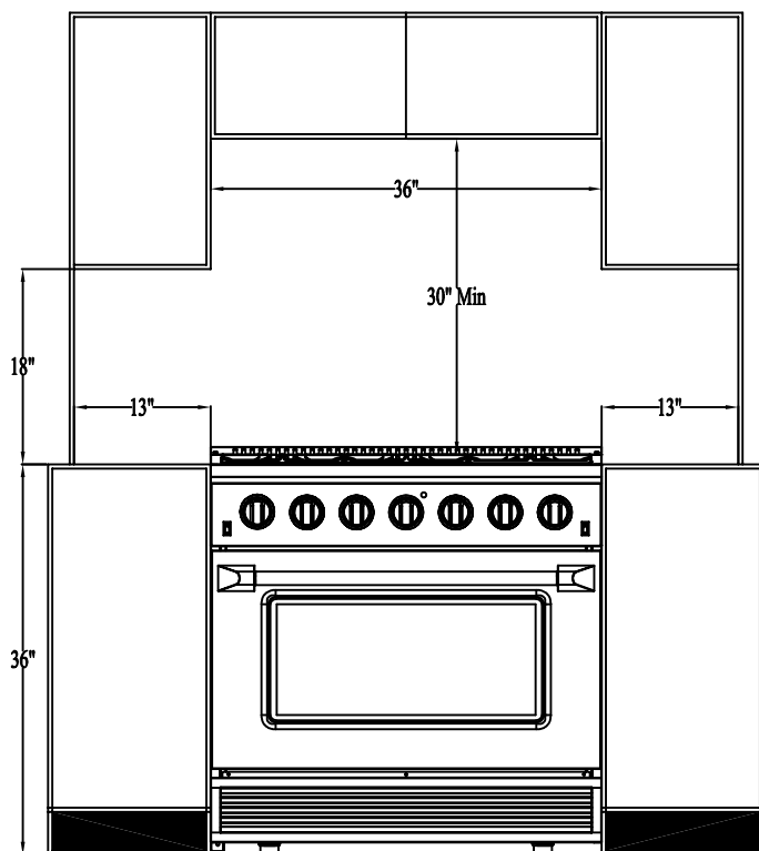
Installation Diagram
