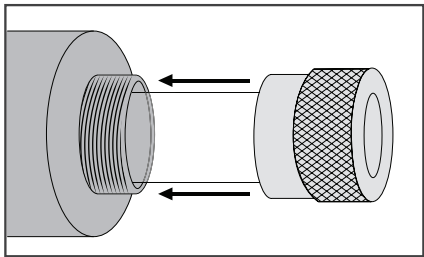
4. Carefully insert the closed end of the Quartz Tube into the open end of the UV Housing with the Metal Cap over the end.
