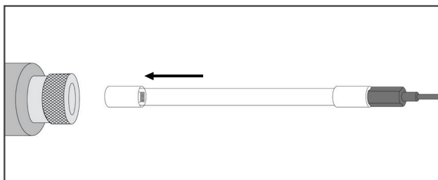
7. Carefully insert the UV Bulb through the opening in the Metal Cap into the Quartz Tube. You will need to remove the housing from its holding clips.
