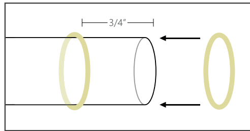
2. Put the O-Ring around the open end of the Quartz Tube (not the bulb) about 3/4 of an inch away from the end.
