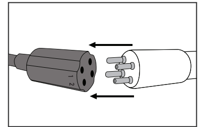
6. Connect the 4 pin electric socket (of the power cord) onto the Ultraviolet Bulb.
