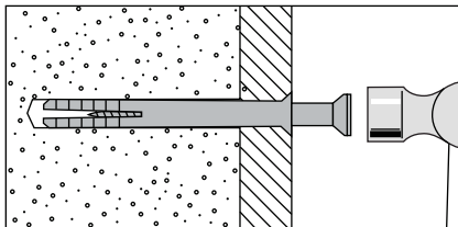
5. Hammer Fixing Wall Plug For use with concrete block or brick walls, or walls stuck with plasterboard. The hammer fixing allows it to be fixed to the wall rather than the plasterboard. Always check the fixing is secure to the retaining wall.
