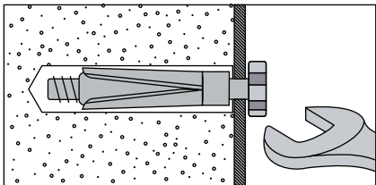
6. Shield Anchor Wall Plug Heavy Loads For use with concrete or brick walls, or for use with heavier loads such as TV & HiFi speakers and satellite dishes, etc.
