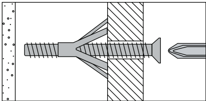
3. Cavity Fixing Wall Plug For use with plasterboard partitions or hollow wooden doors.
