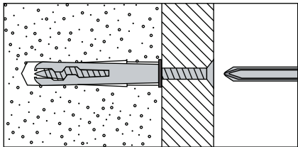
1. General Purpose Wall Plug Generally, aerated blocks should not be used to support heavy loads, use a specialist fitting in this case. For light loads, general purpose wall plugs can be used.
