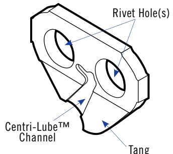
DRIVE LINK
