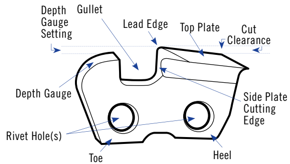
CUTTER TOOTH
