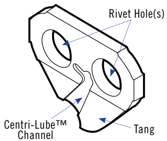
DRIVE LINK
