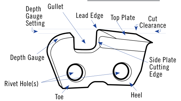
CUTTER TOOTH
